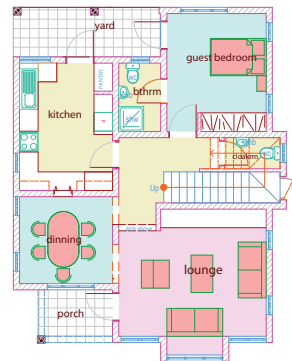
MAISONNETTE GROUND FLOOR PLAN
