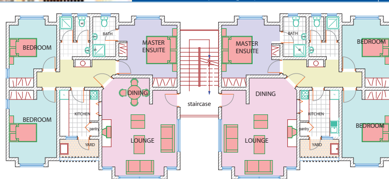
APARTMENTS TYPICAL FLOOR PLAN
